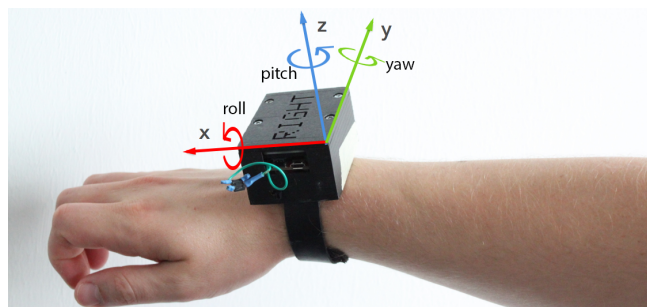
Figure 5. Sensor box attached to wrist. The attached button is used to manually mark timestamps in the recorded data. The x-axis runs parallel to the arm which is later used to determine if the arm is pointing up- or downward. Yaw, pitch, and roll corresponds to the y-, z-, and x-axis.
