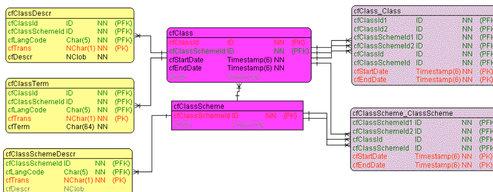
Figure 3: CERIF Semantic Layer in ERM physical view*
