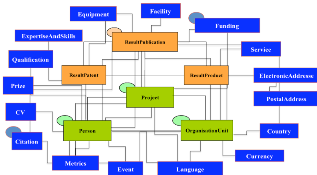
Figure 1: CERIF Entities and their Relationships in abstract view
