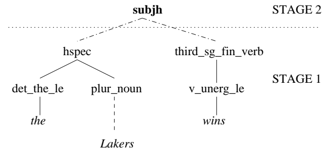
Figure 2: An example of pseudo-derivation tree in a two-stage robust parsing model
