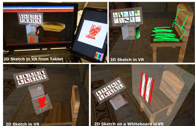
Figure 1: We consider 4 different interaction methods in virtual environments:(top-left) 2D sketching on a real tablet, (top-right) 3D mid-air sketching, (bottom-left) 2D sketching on a virtual tablet and (bottom-right) 2D sketching on a fixed virtual whiteboard.
