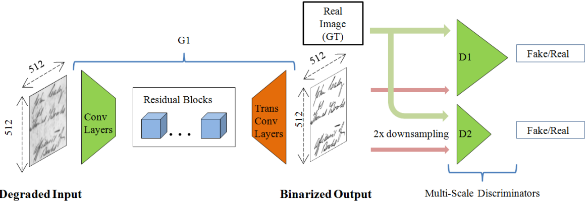
Figure 3: Global network with Convolution Layers, Residual Blocks and Transpose-Convolution Layers as Generator \{G1\} and Multi-Scale Discriminators D1 and D2, which work at 512 X 512 and 256 X 256 respectively.
