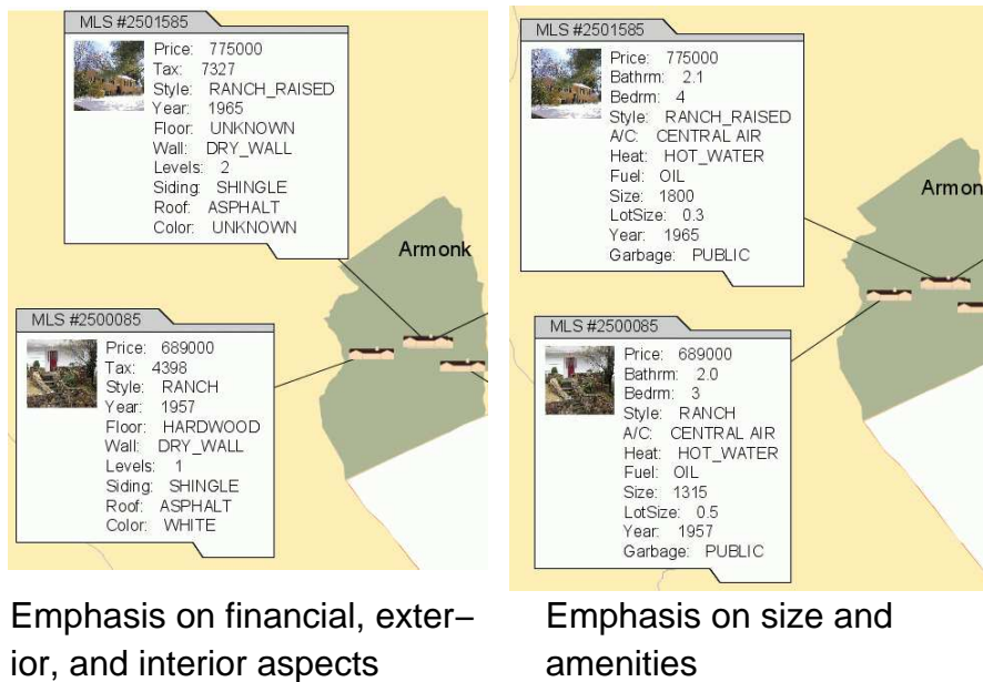
Figure 22.17. Two cropped screen shots from the RIA multimedia conversation system. (Screen shots courtesy of Vikram Aggarwal.)
