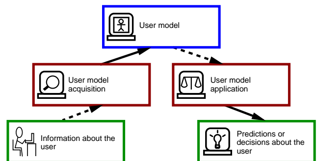
Figure 22.2. General schema for the processing in a user-adaptive system. (Dotted arrows: use of information; solid arrows: production of results.)
