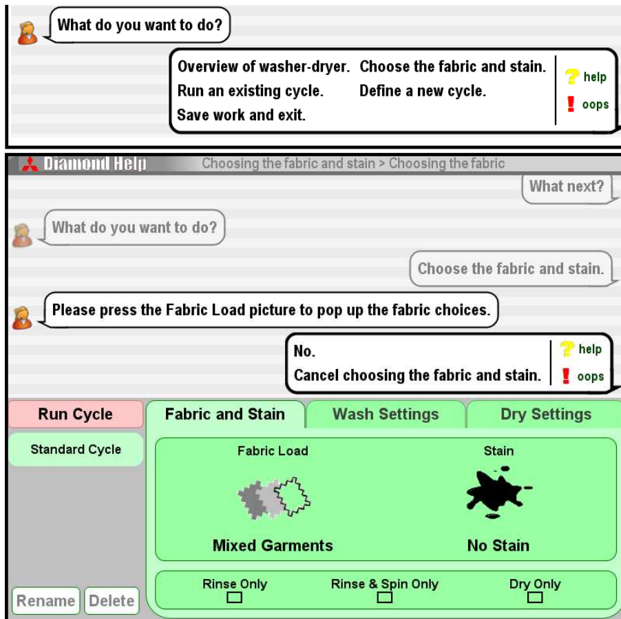
Figure 22.8. Example of collaborative assistance offered by DIAMONDHELP. (Explanation in text. Screen shots courtesy of Charles Rich.)
