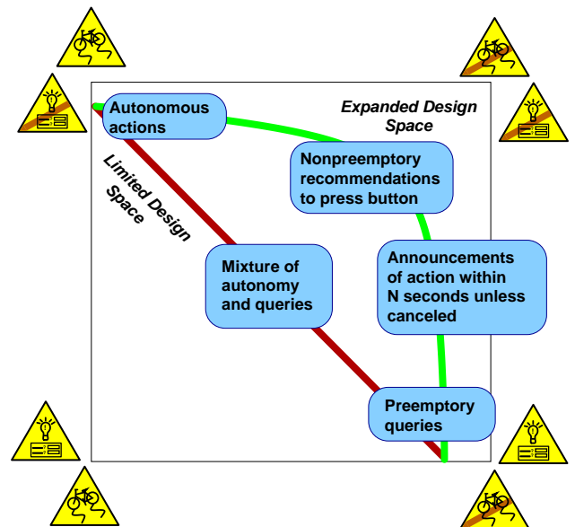
Figure 22.24. Illustration of strategies for dealing with tradeoffs among usability goals in user-adaptive systems. (Explanation in text.)
