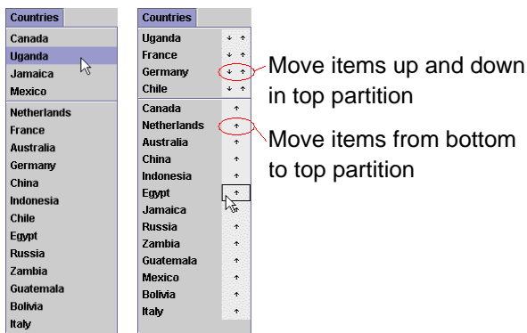
Figure 22.27. The adaptive (left) and adaptable (right) split menus used in an experimental comparison. (Adapted from Figure 1 of “A comparison of static, adaptive, and adaptable menus,” by L. Findlater & J. McGrenere, 2004, in E. Dykstra-Erickson & M. Tscheligi (Eds.), Human factors in computing systems: CHI 2004 conference proceedings , pp. 89–96, New York: ACM, Copyright 2004 by the Association for Computing Machinery, Inc. Adapted with permission.)
