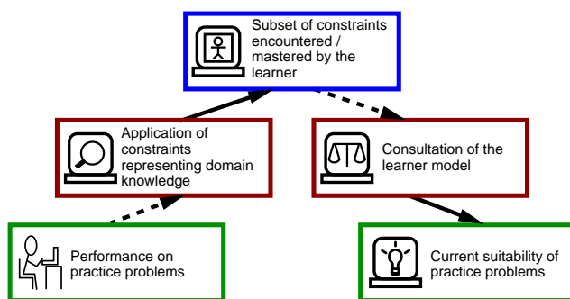
Figure 22.22. Overview of adaptation in the SQL Tutor.
