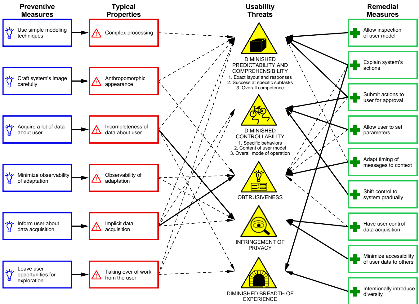
Figure 22.23. Overview of usability challenges for user-adaptive systems and of ways of dealing with them. (Dashed arrows denote threats and solid arrows mitigation of threats, respectively; further explanation is given in the text.)
