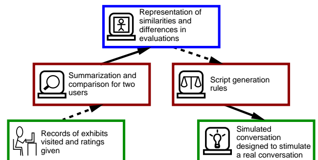
Figure 22.20. Overview of adaptation in AGENTSALON.
