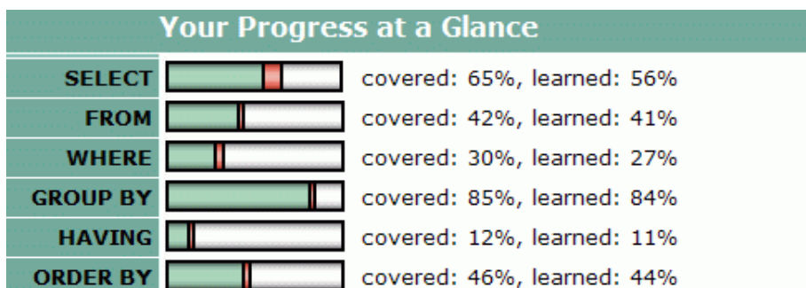
Figure 22.21. Screen shots from the SQL-TUTOR. (Above: the main interface; below: display of the learner model. Screen shots courtesy of Antonija Mitrovic.)
