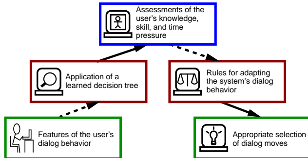
Figure 22.13. Overview of adaptation in KYOTO CITY BUS INFORMATION SYSTEM.
