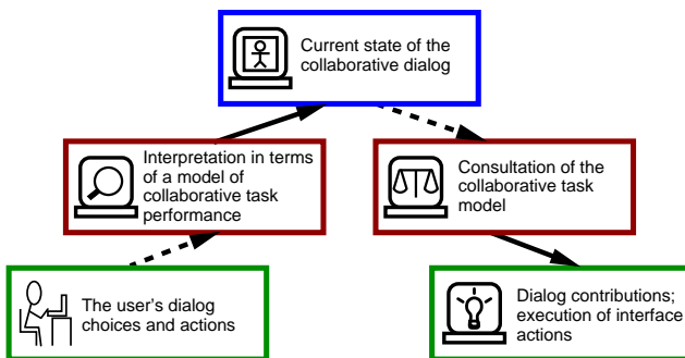
Figure 22.9. Overview of adaptation in DIAMONDHELP.
