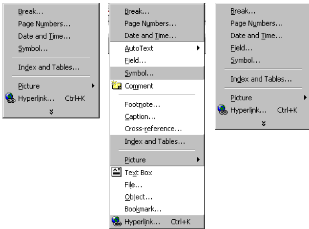
Figure 22.6. Example of adaptation in SMART MENU. (The user accesses the “Insert” menu. Not finding the desired option, the user clicks on the extension arrows and selects the “Field” option. When the user later accesses the same menu, “Field” now appears in the main section.)
