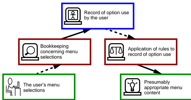
Figure 22.7. Overview of adaptation in SMART MENU.
